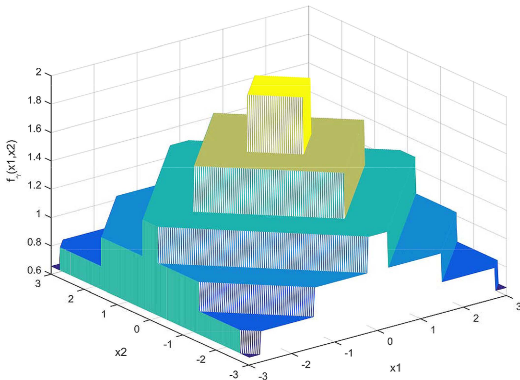
Two dimensional Staircase-Shaped Probability Density Function for Differential Privacy. For more see "The Staircase Mechanism in Differential Privacy" by Q. Geng, et al. , p. 1176.
